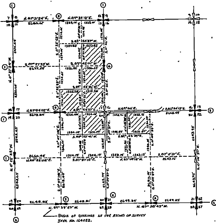
SECTION BREAKDOWN SKETCH N.T.S.
